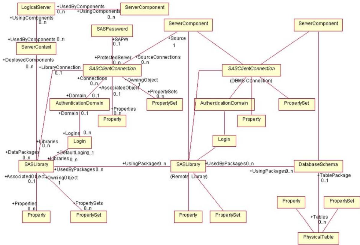
Figure 4.3 Remote Relational DBMS Model
